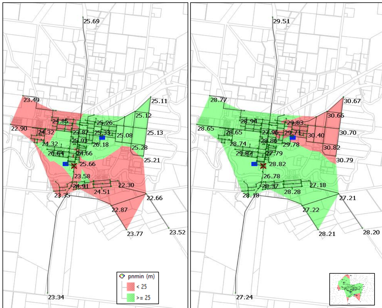
Appendix Figure G.5-3: Potable WSS Upgrade Option 1 - Pressure contours (L: minimum pressure and R: maximum pressure)
