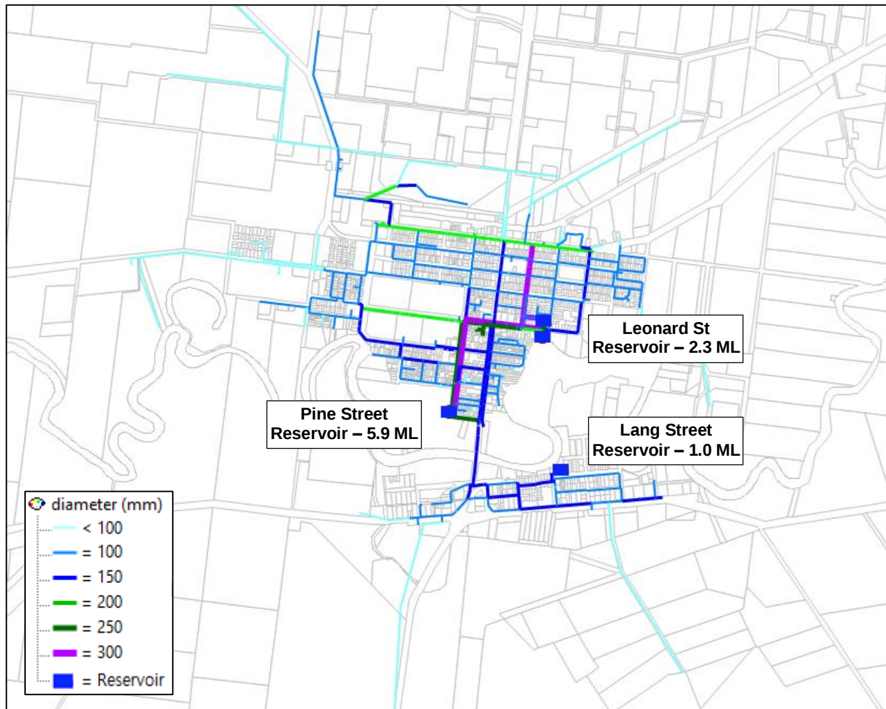
Figure 2-7: Hay raw water reticulation system layout plan
